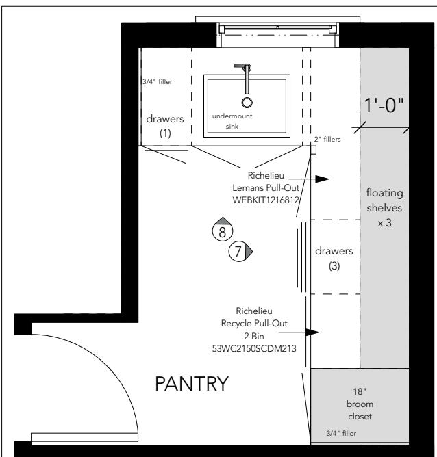
PANTRY PLAN SCALE: 3/8" = 1'-0"
