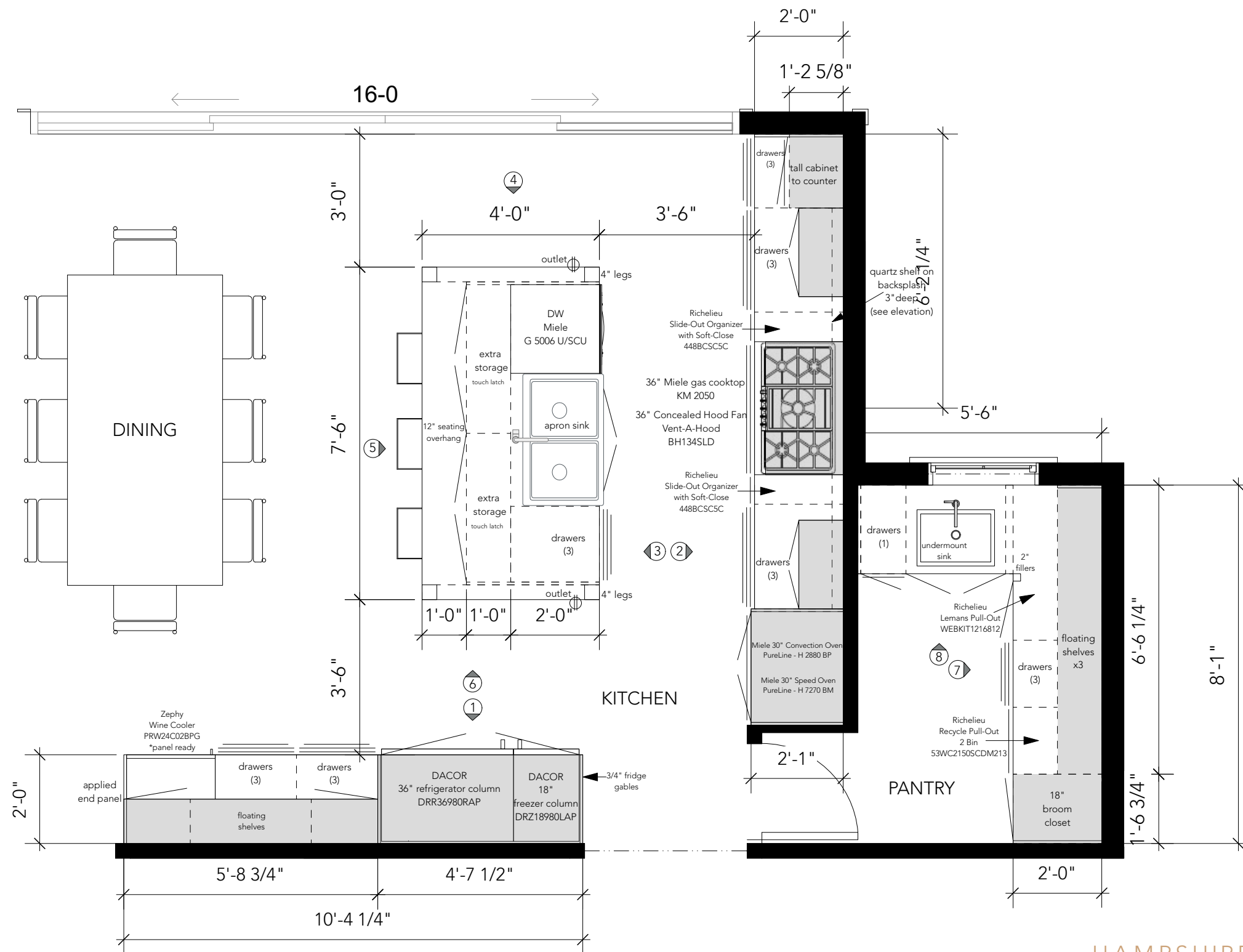
KITCHEN PLAN SCALE: 3/8" = 1'-0"
