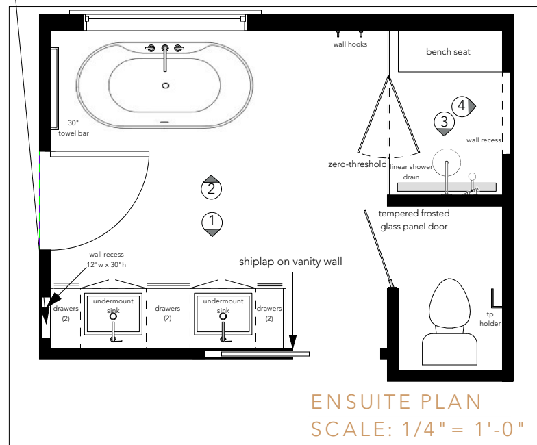
WALL RECESS 12"w x 30"h
