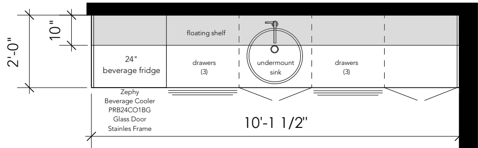
CABINETRY PLAN SCALE: 3/8" = 1'-0"
