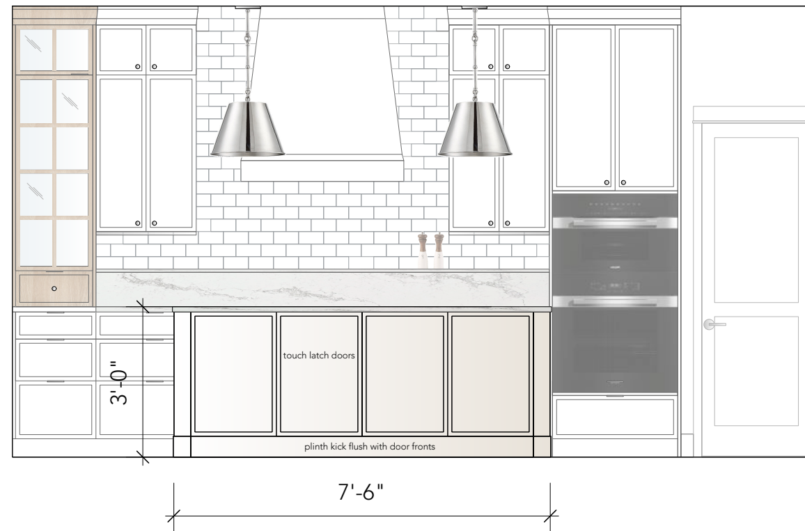
ISLAND ELEVATIONS SCALE: 3/8" = 1'-0"
