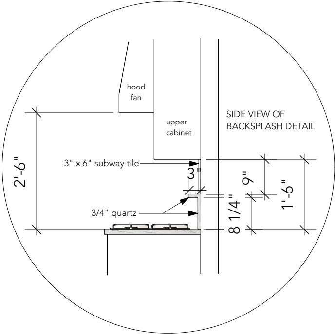
BACKSPASH DETAIL
