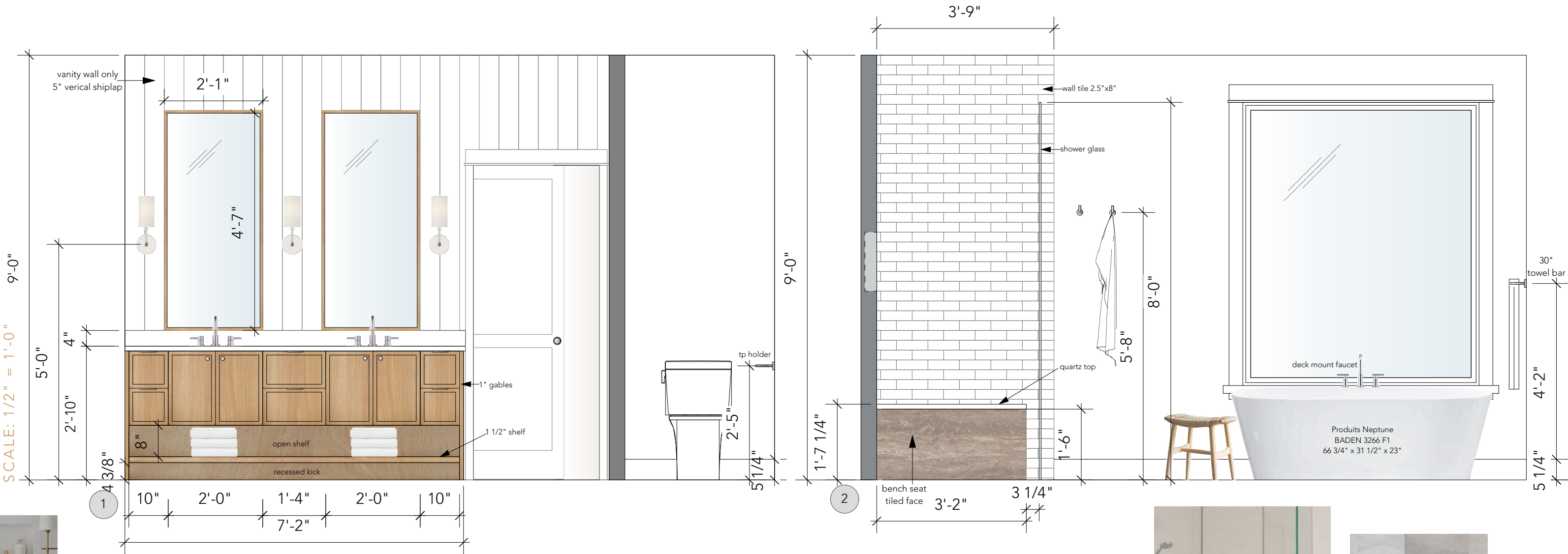
WALL RECESS 12" w x 30" h
