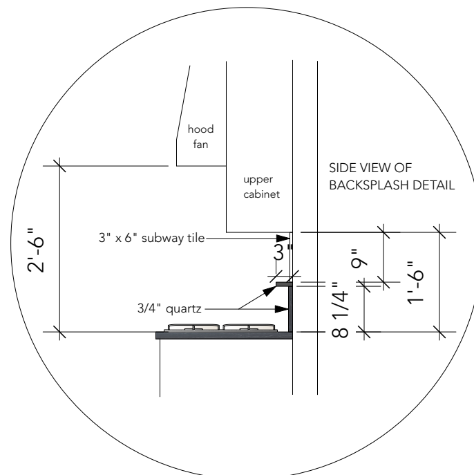
BACKSPLASH DETAIL
