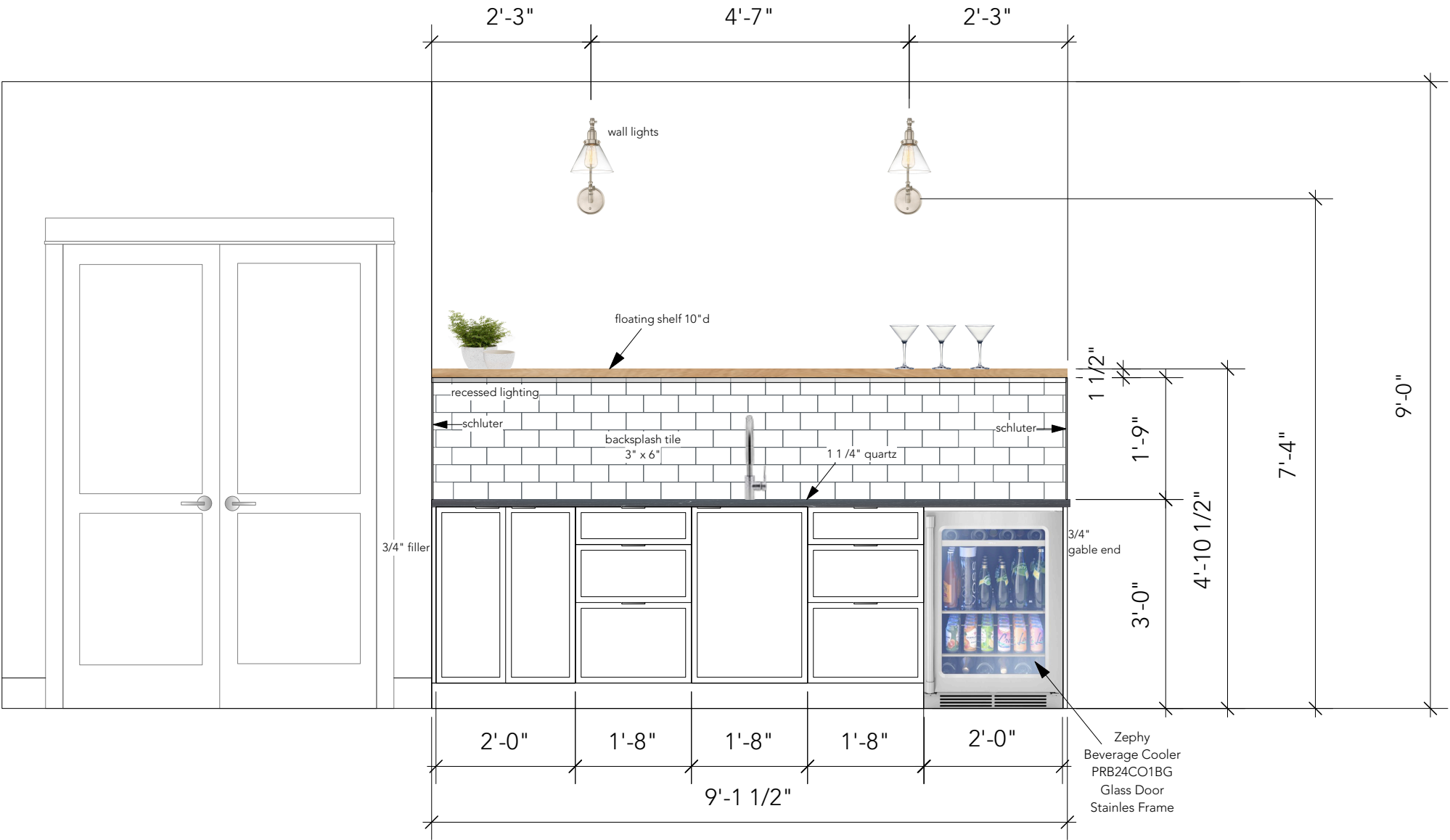
LOWER FLOOR BAR ELEVATION SCALE: 1/2" = 1'-0"
