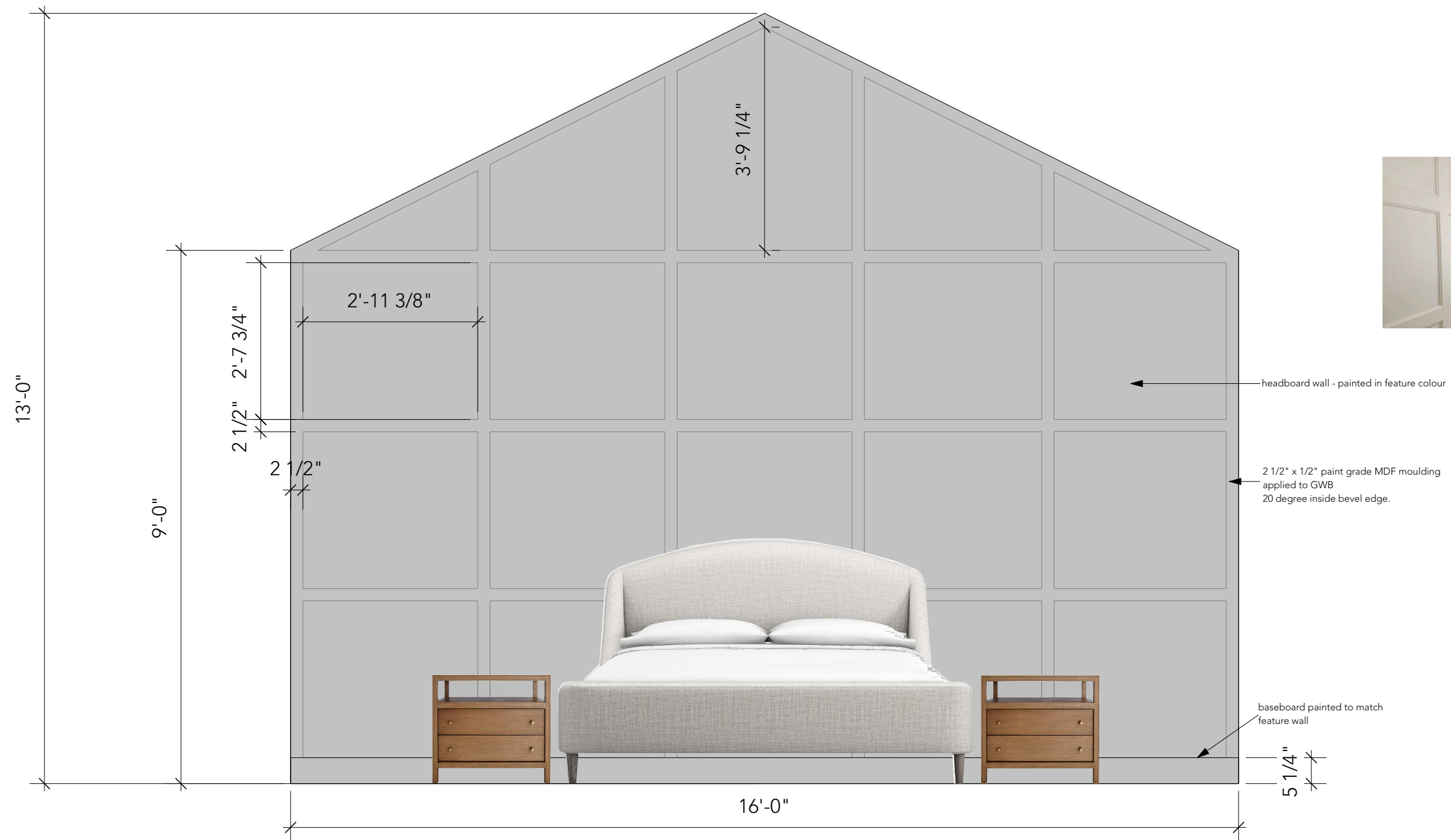
HEADBOARD MOULDING DETAIL - painted feature colour
