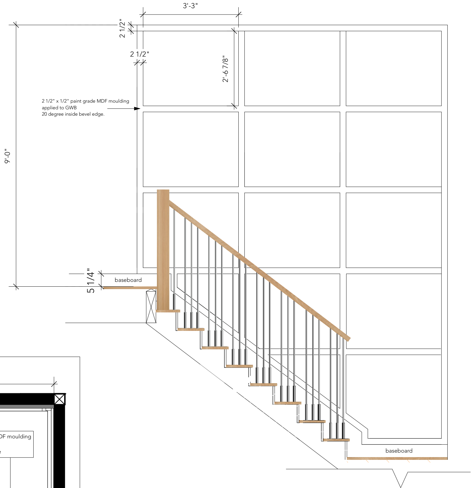
SECOND FLOOR STAIR WALL ELEVATION SCALE: 1/2" = 1'-0"
