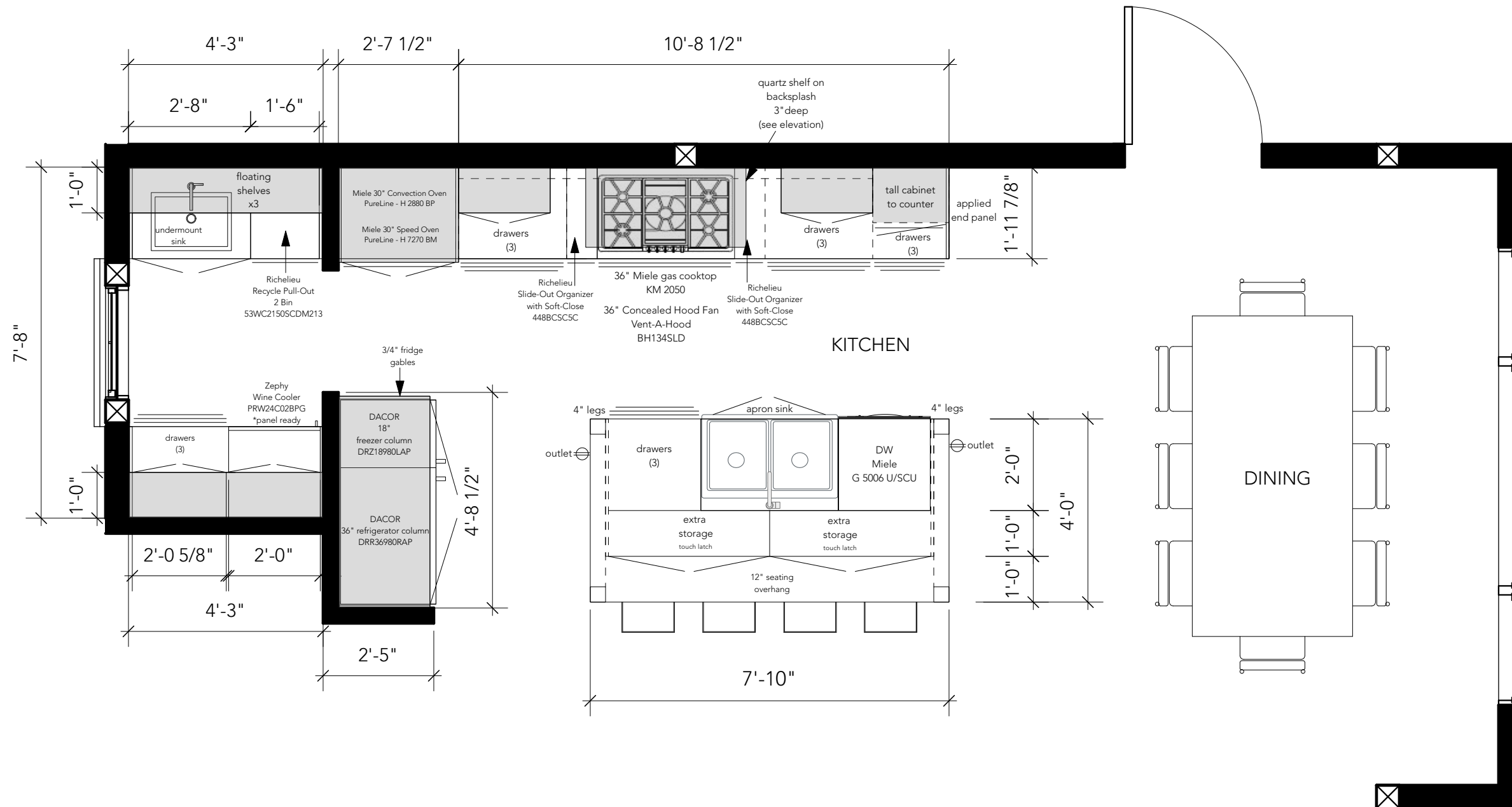
KITCHEN PLAN SCALE: 3/8" = 1'-0"
