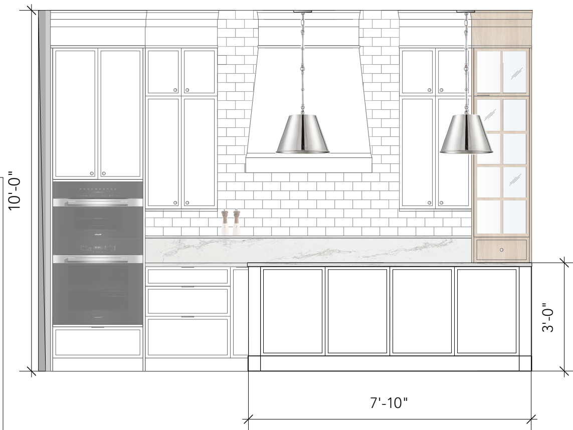
ISLAND ELEVATIONS SCALE: 3/8"=1'-0"
