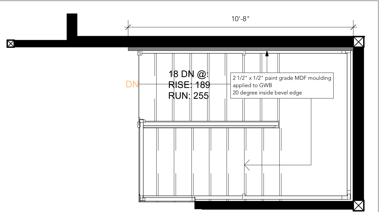
SECOND FLOOR STAIR WALL SCALE: 3/8" = 1'-0"
