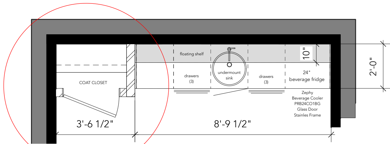
LOWER FLOOR BAR PLAN SCALE: 3/8" = 1'-0"
