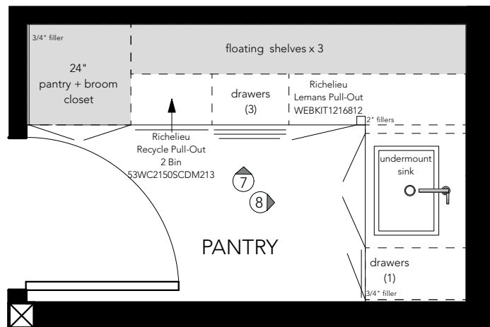
PANTRY PLAN SCALE: 3/8" = 1'-0"
