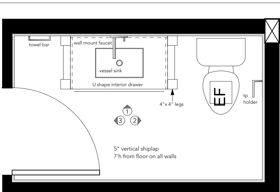
POWDER ROOM PLAN SCALE: 1/2" = 1'-0"
