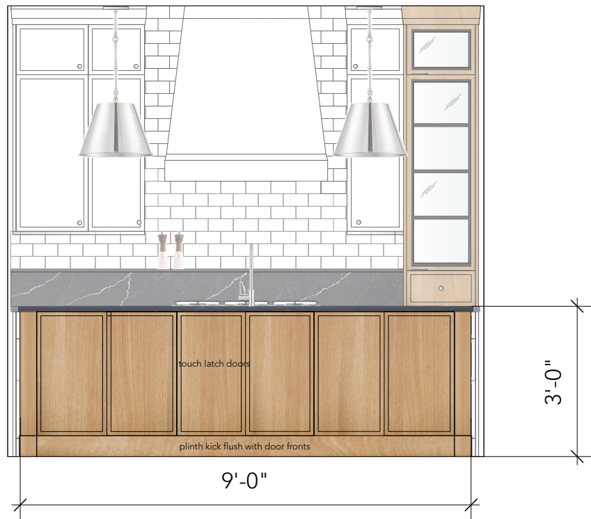
ISLAND ELEVATIONS SCALE: 3/8" = 1'-0"
