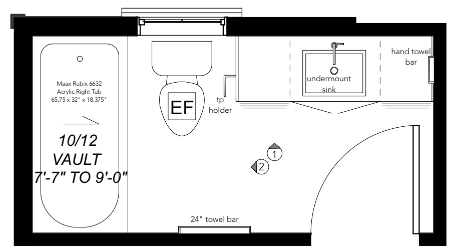
SECOND FLOOR GUEST ENSUITE 3 SCALE: 3/8" = 1'-0"
